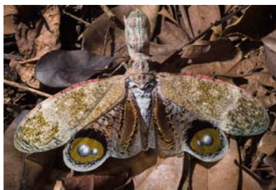
Fulgoridae Fulgora laternaria
